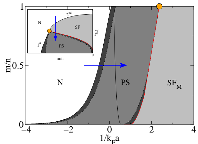
FIG. 1: (Colour online) Zero temperature mean-field phase diagram for magnetisation m/n versus interaction strength 1/k_F a . The phase separated region (PS) can be decomposed into two regions — the spinodal or unstable region and the metastable region (darker shade) — divided by the spinodal normal (sp-N) line (dashed) and the spinodal superfluid (sp-SF) line (dot-dashed). In addition, the PS spinodal phase is divided in half by the line where the superfluid density Q is zero (thin solid). The tricritical point (orange circle) is at m/n = 1 and 1/k_F a \simeq 2.37 . Inset: schematic finite temperature phase diagram of T_c/\varepsilon_F versus m/n for a fixed interaction strength 1/k_F a . Arrows indicate possible quenches into the spinodal region.
